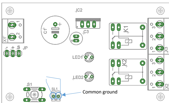
Connectors layout on board SVR v1.2
